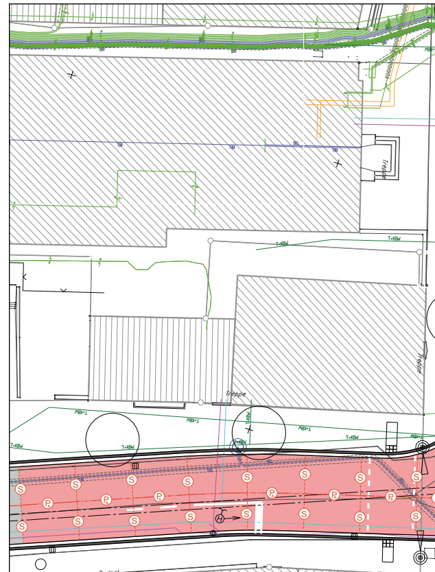
Abb. 11: Betonfugenplan
